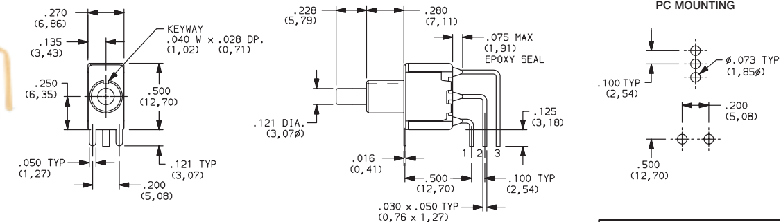
8121SD9AVGE SPDT
