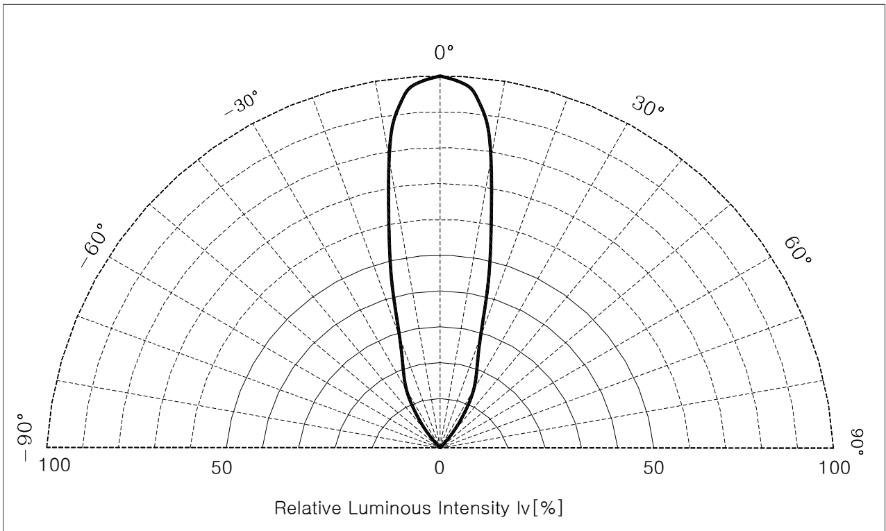
Fig. 5 Radiation Diagram
