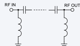
schematic B
