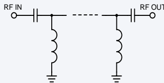
schematic A
