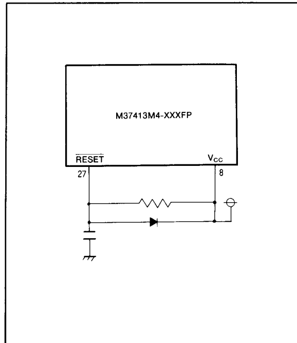
Fig. 18 Example of reset circuit
