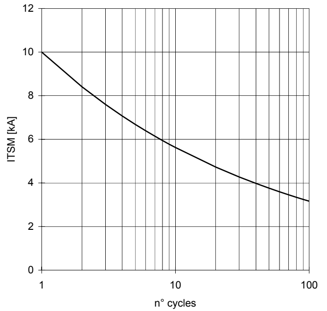
SURGE CHARACTERISTIC T_j = 120\text{ }^\circ\text{C}
