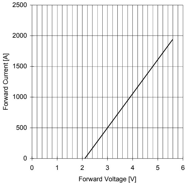
FORWARD CHARACTERISTIC T_j = 120\text{ }^\circ\text{C}
