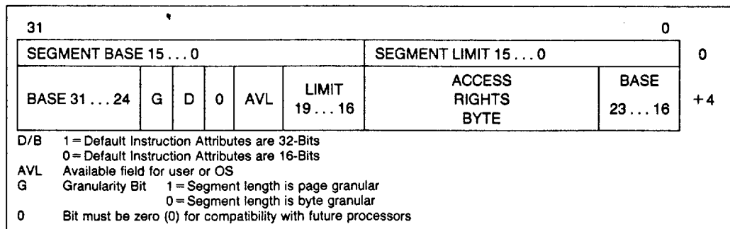
Figure 4.6. Segment Descriptors
