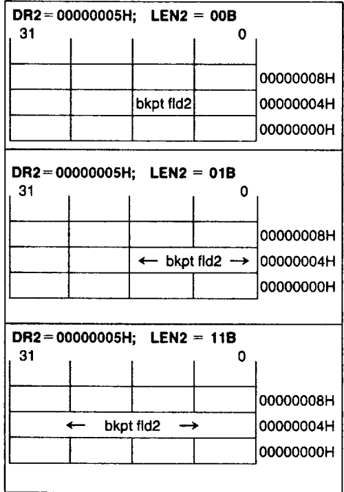
Figure 9.1. Debug Registers
