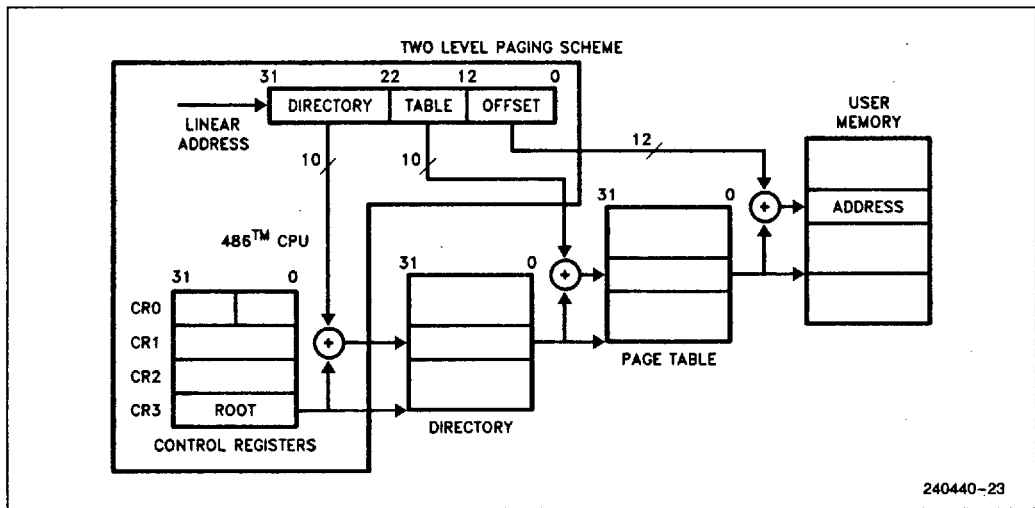
Figure 4.19. Paging Mechanism
