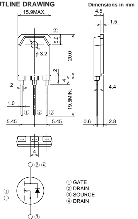
TO-3P
