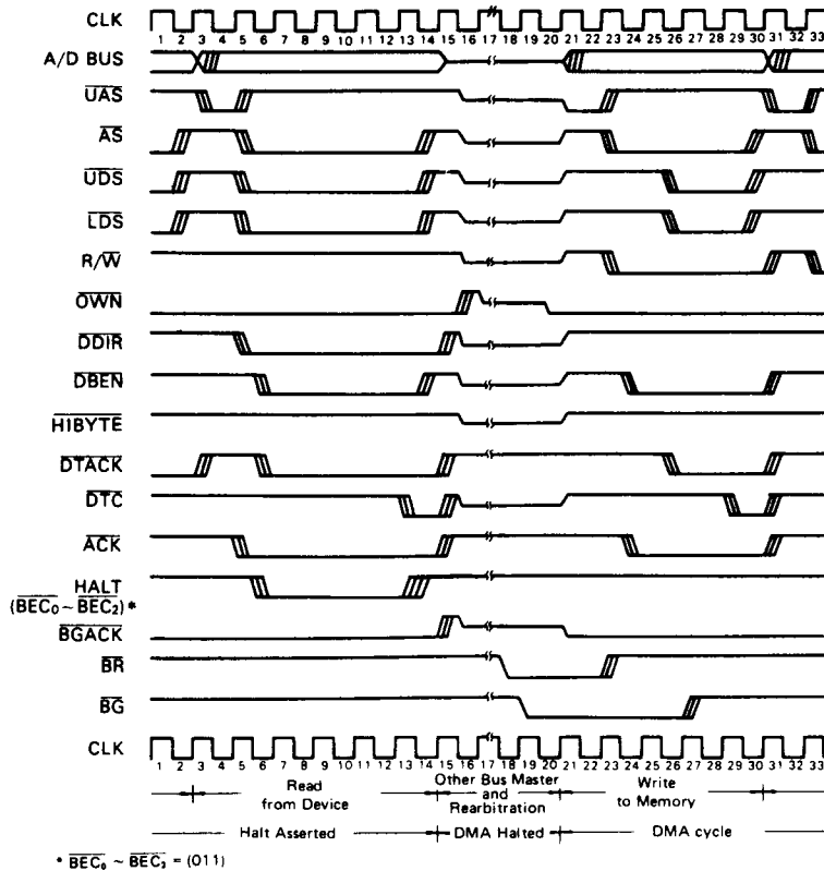
Figure 39 Halt Operation
