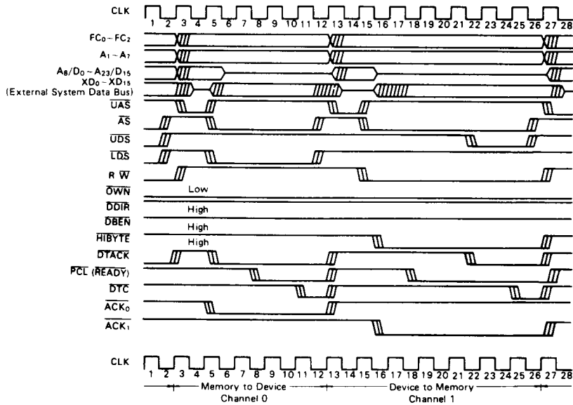
Figure 35 Single Addressing Mode with 8-Bit Devices as Source and Destination with PCL Used as a \overline{READY} Input (Read-Write Cycles)
