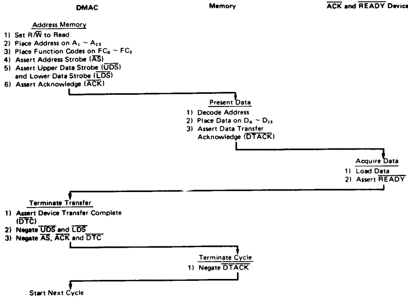
Figure 33 Word from Memory to Device with ACK and READY
