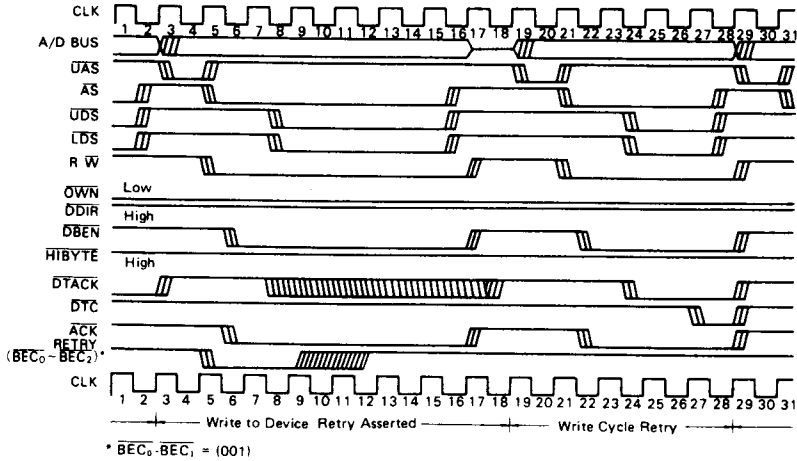
Figure 41 Retry Operation
