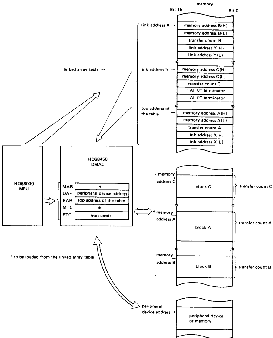
Figure 3B Transfer Example of the Linked Array Chaining Mode
