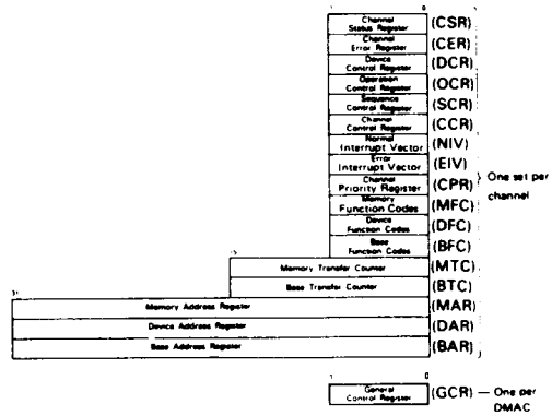
Figure 10 Internal Registers
