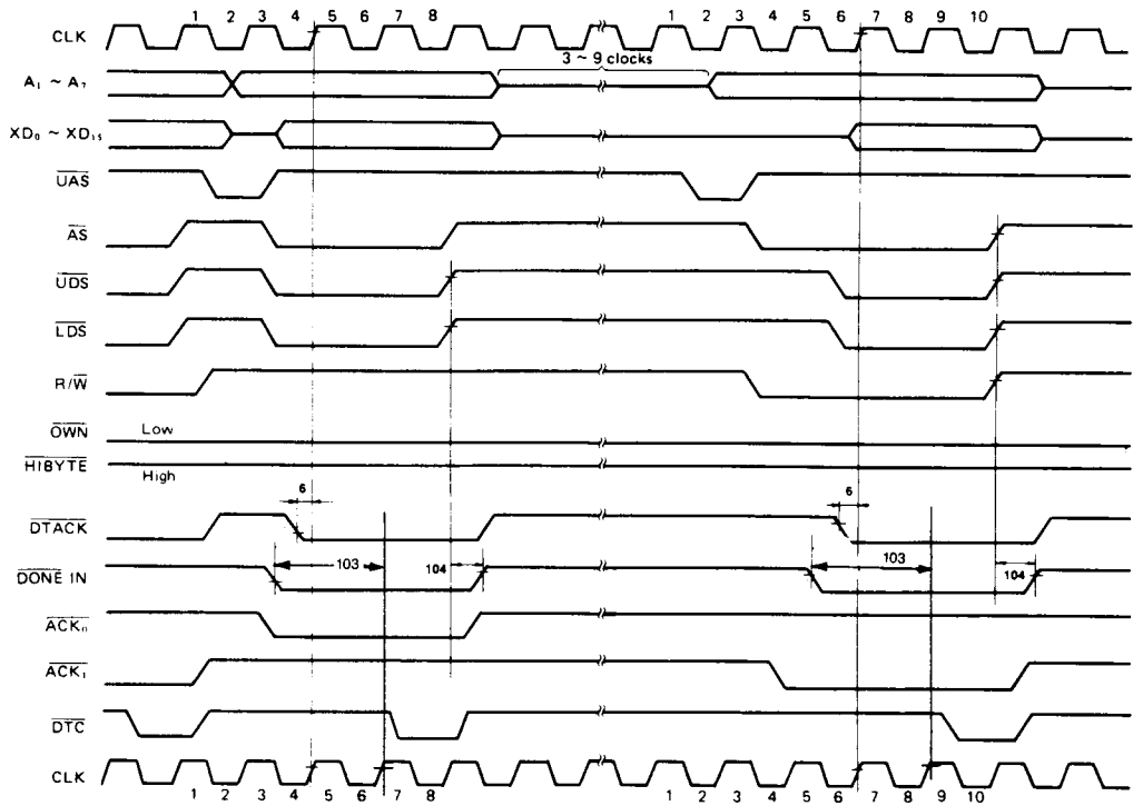
Figure 8 AC Electrical Waveforms – \overline{D0NE} Input
