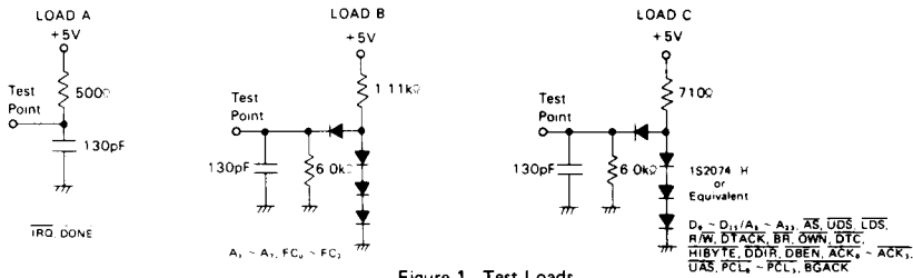
Figure 1 Test Loads
