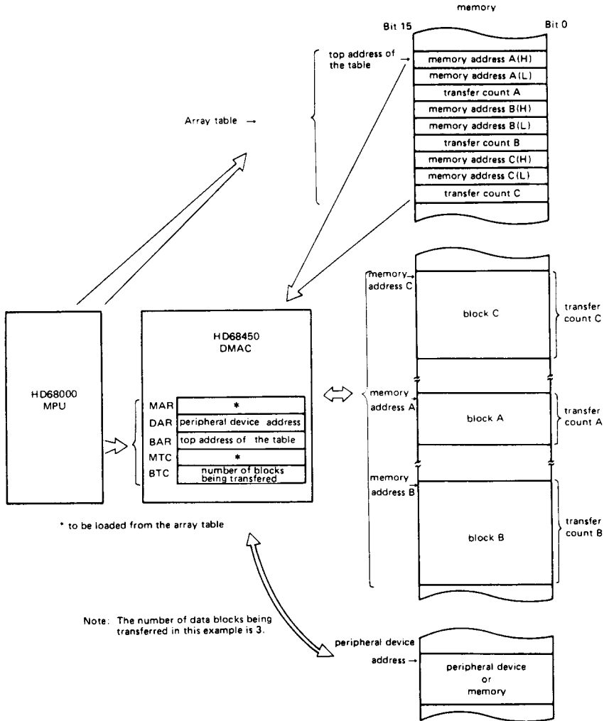
Figure 37 Transfer Example of the Array Chaining Mode
