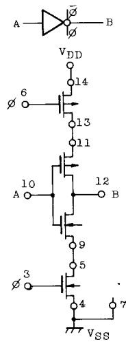
2. CLOCKED INVERTER
