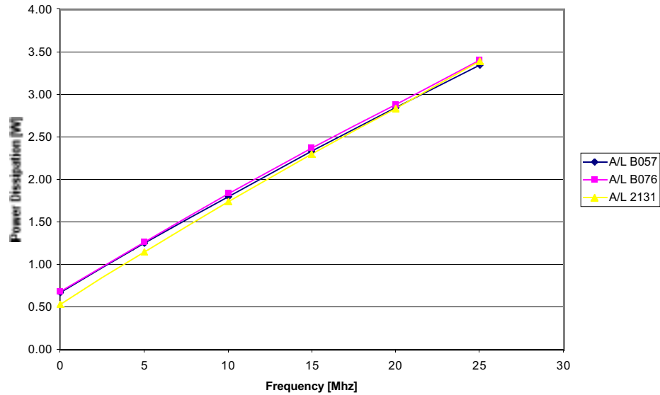
Figure 6. Edge818 Power Dissipation vs. Operating Frequency (VCC = 12V, VEE = -3.3V, VH = 3.3V, VL = 0V, Zload = 1KΩ||80pF, Ta = 25 °C, Airflow = 300 LFPM, All 8 Driver Channels Toggled)
