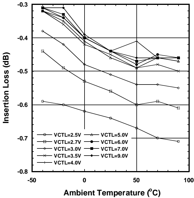
Insertion Loss vs. Ambient Temperature
