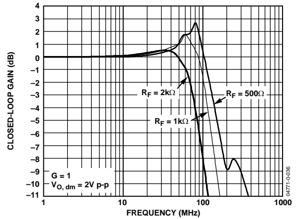
Figure 22. Large Signal Frequency Response for Various R_f
