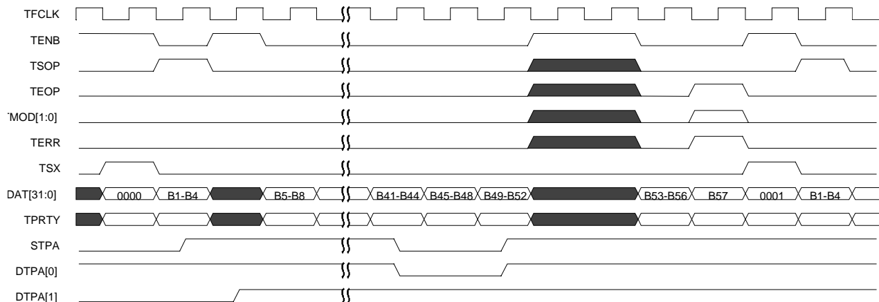
Figure 6.1: Transmit Logical Timing
