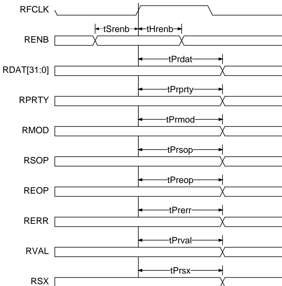
Figure 7.4: Receive Physical Timing
