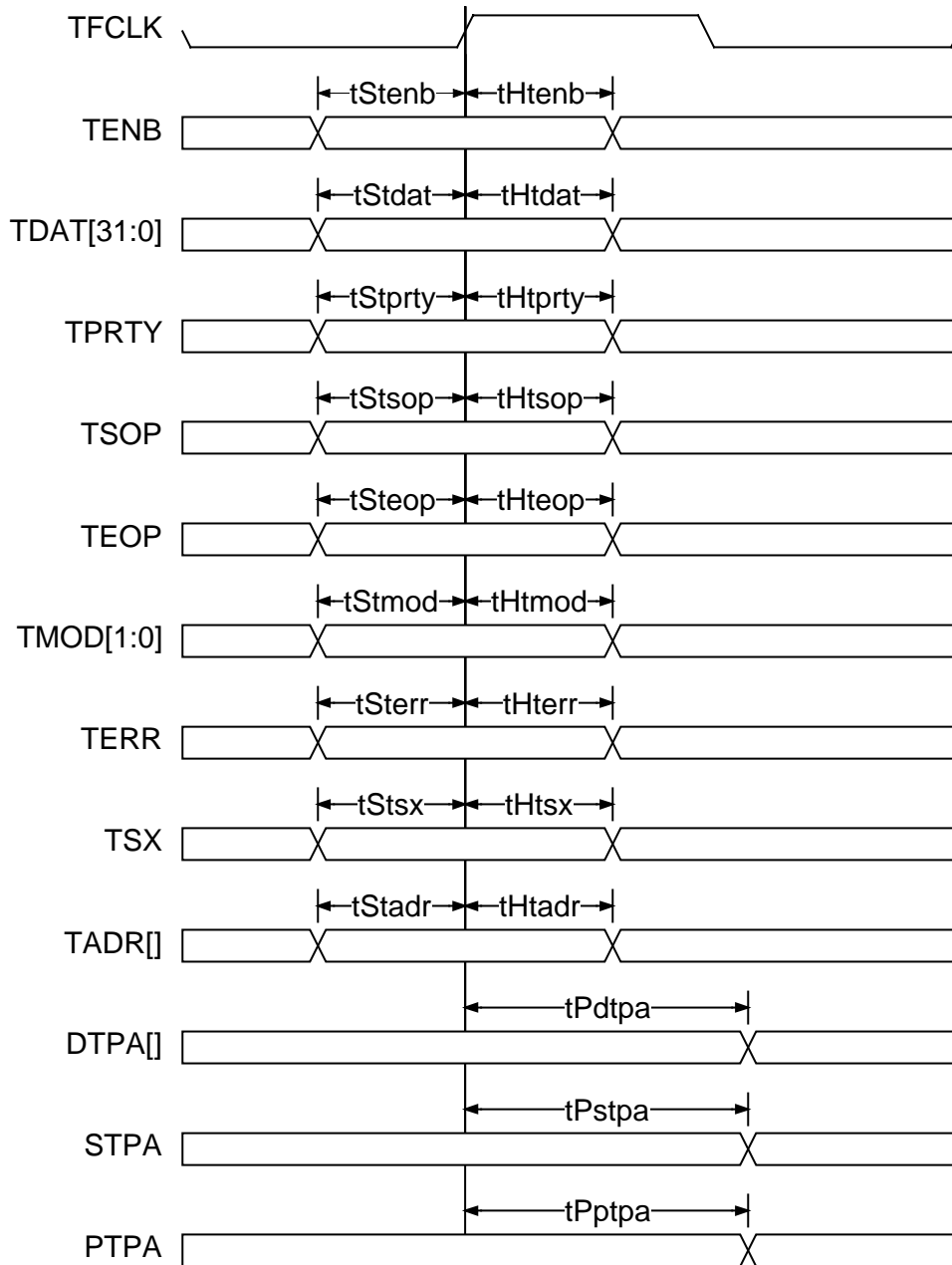
Figure 6.3. Transmit Physical Timing
