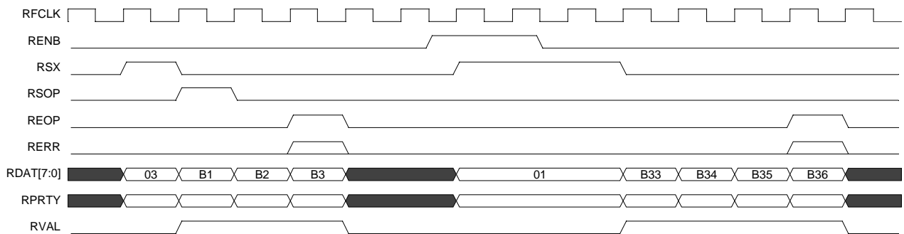
Figure 7.2: Receive Logical Timing with Pausing
