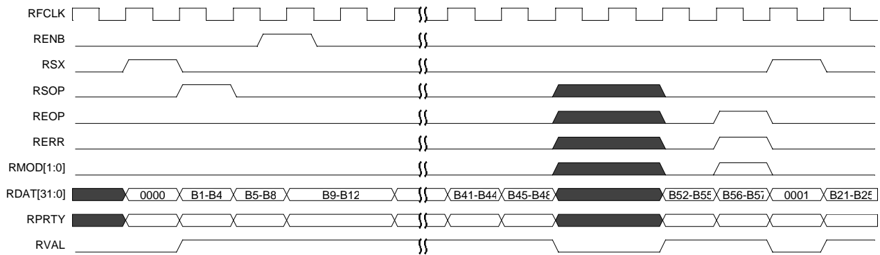
Figure 7.1: Receive Logical Timing
