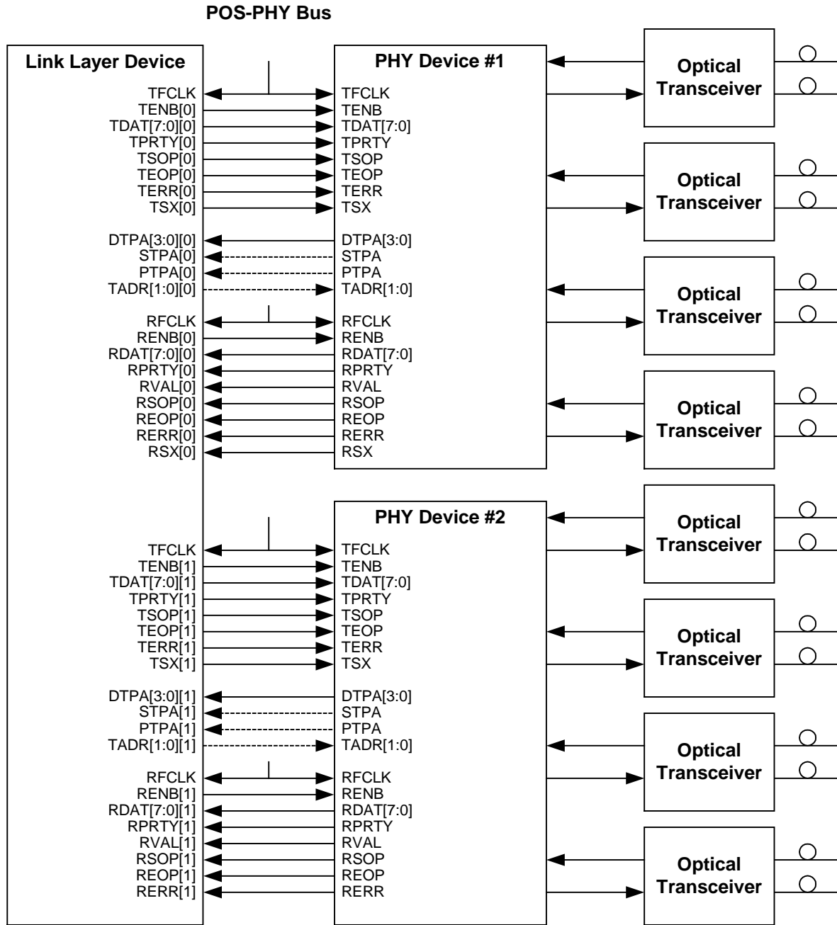
Figure 4.2: POS-PHY PHY to Link Layer 8-Bit Interface
