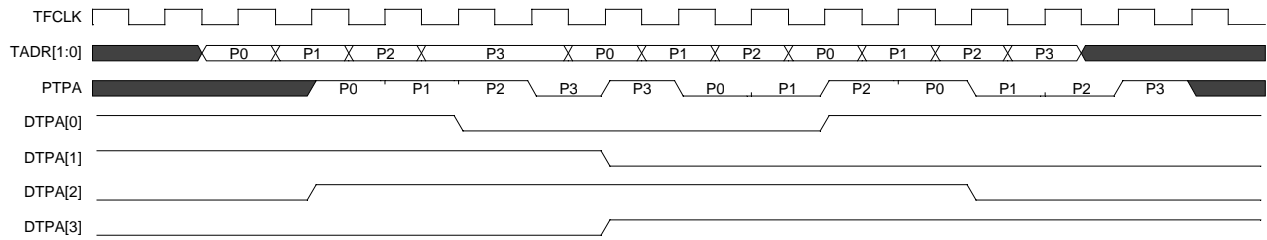
Figure 6.2: Packet-Level Transmit Polling Logical Timing
