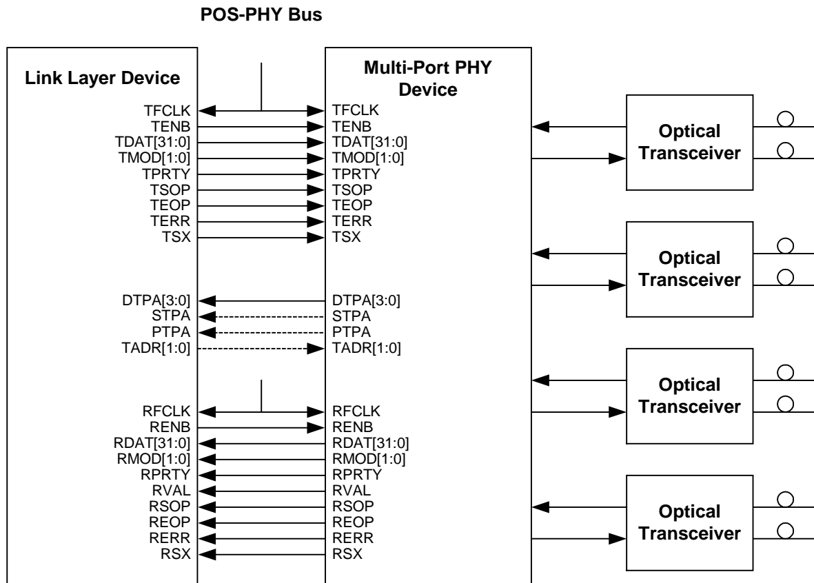
Figure 4.1: POS-PHY PHY to Link Layer 32-bit Interface
