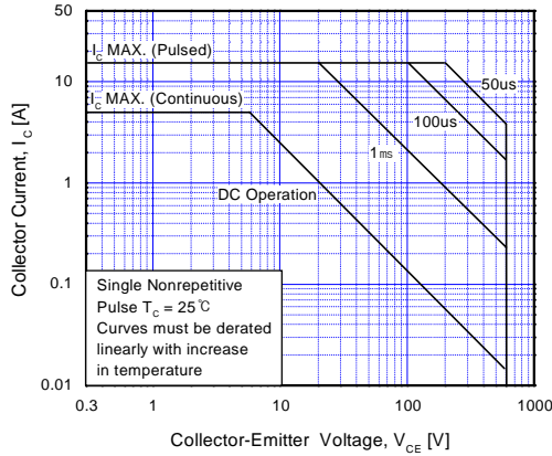
Fig 15. SOA Characteristic
