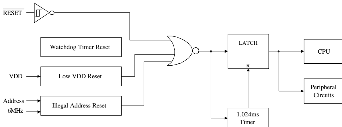
Fig. 1 Reset Signals
