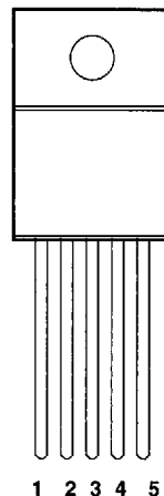
TO-220-5 Package (MIC29201/29202/29203BT)
