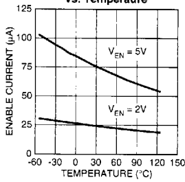
MIC29201/2 Shutdown Current vs. Temperature
