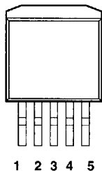
TO-263-5 Package (MIC29201/29202/29203BU)
