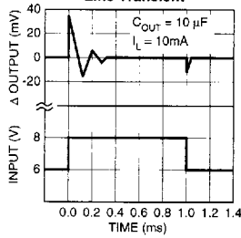
Line Transient
