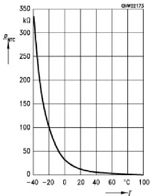
NTC Thermistor R_T = f(T_A) R_{T=25^\circ C} = 10\text{ k}\Omega \pm 1\%
