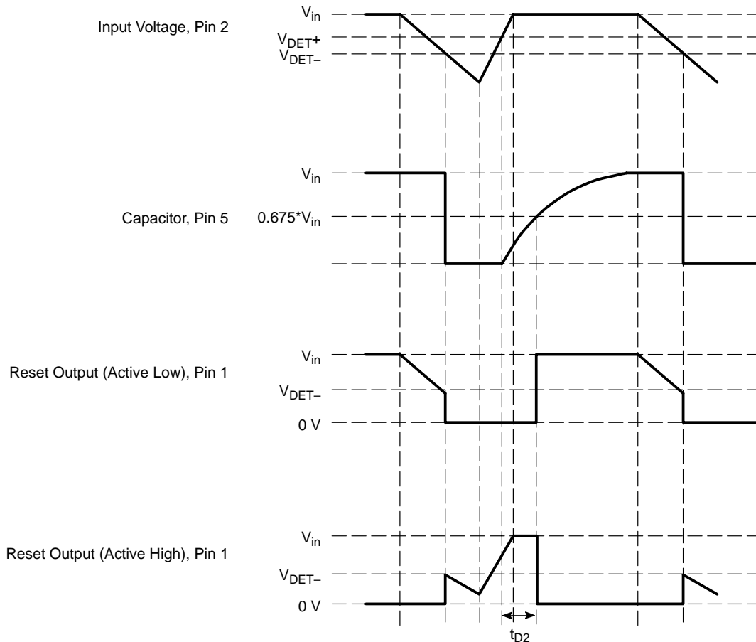
Figure 36. Timing Waveforms
