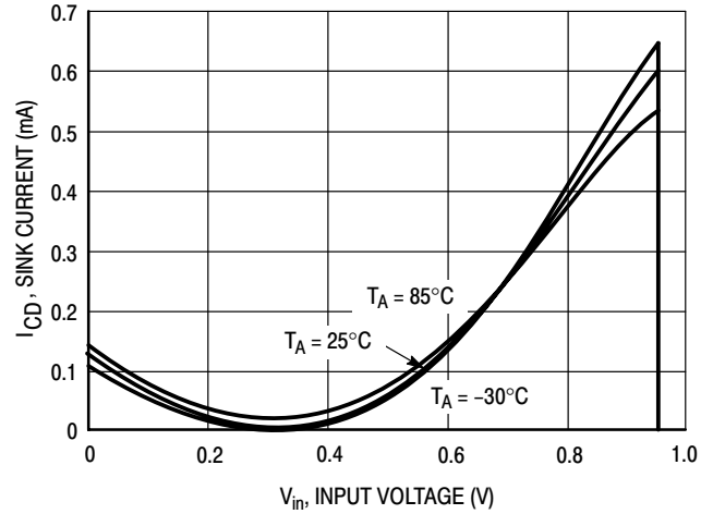
Figure 29. NCP302/3 Series 0.9 V C D Pin Sink Current versus Input Voltage
