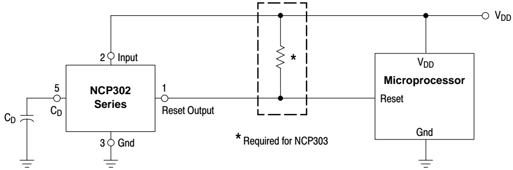
Figure 37. Microprocessor Reset Circuit (NCP302 and NCP303 Series)
