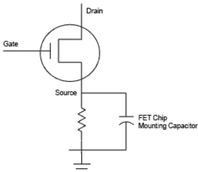
Figure 2. Schematic Diagram
