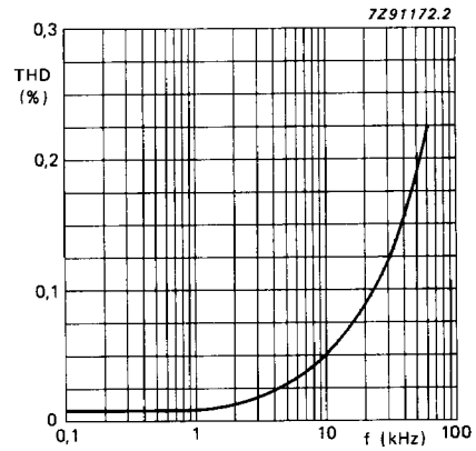
Fig. 5 Total harmonic distortion (THD) as a function of operating frequency ( f ); V_p = 33 V; R_L = 4 Ω; P_O = 10 W (constant).
