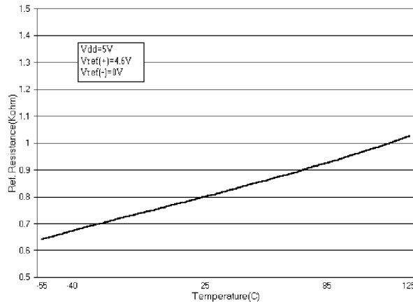
Graph 9. Reference Resistance vs. Temperature
