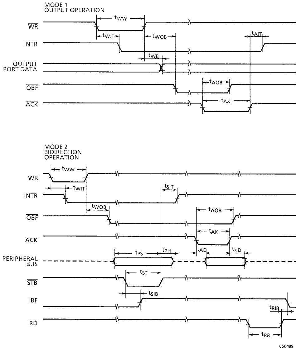
Figure 7.2 Timing Diagram
