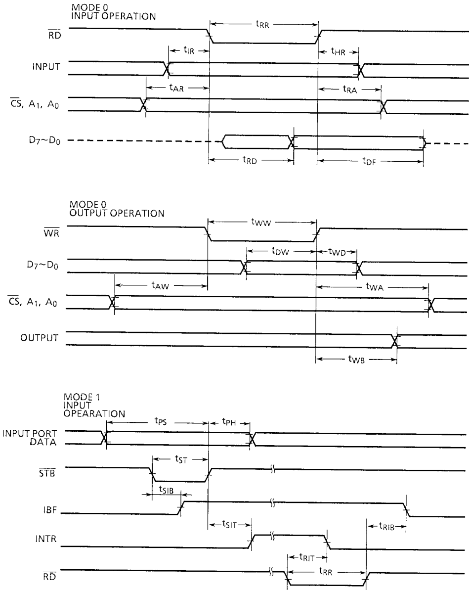
Figure 7.1 Timing Diagram
