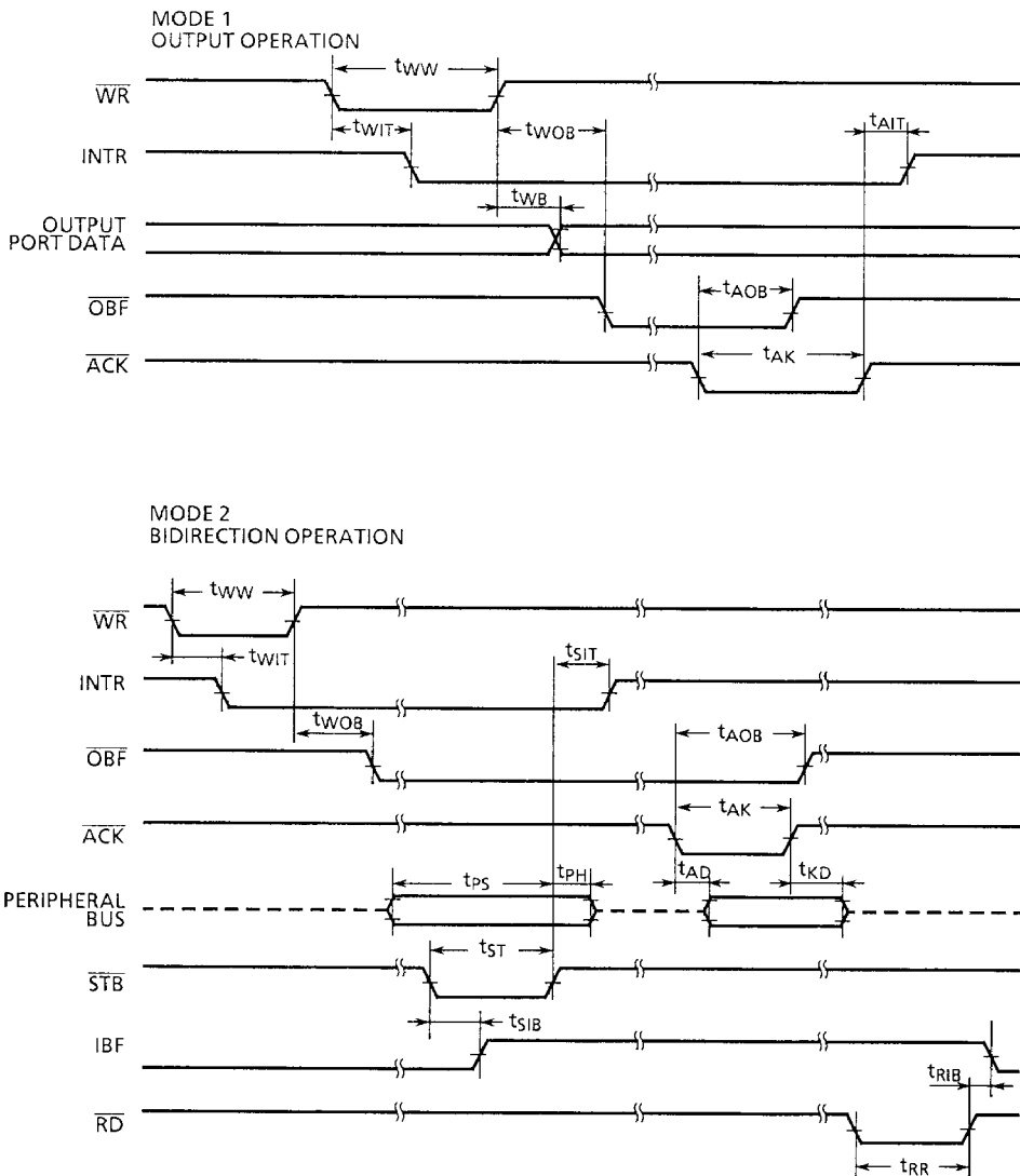
Figure 7.2 Timing diagram
