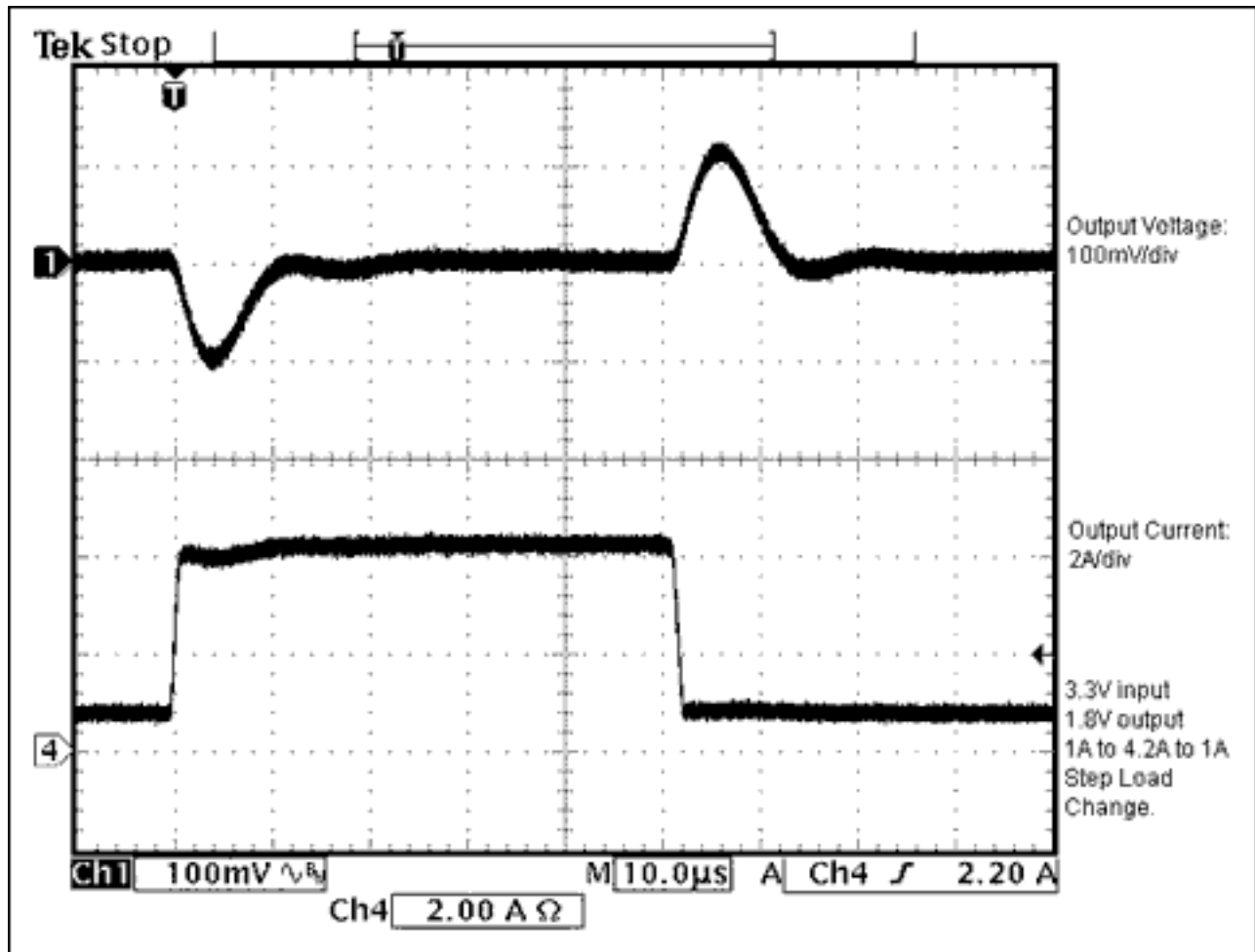
Figure 3. Step load transient response: output current from 1A to 4.2A back to 1A. The output voltage back to regulation within 10 \mu s for 50% step load change.
