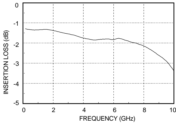
Insertion Loss
