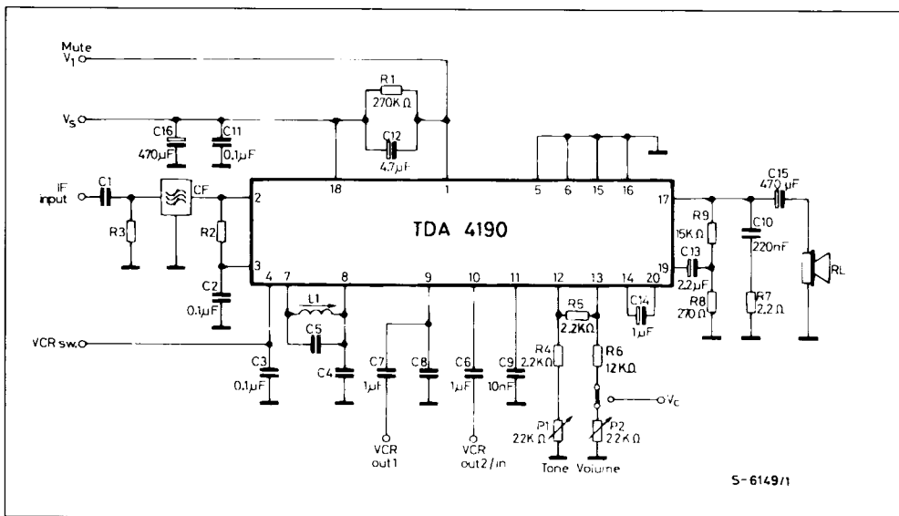
Figure 16 : Application Circuit.
