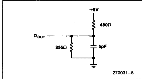
Load B
