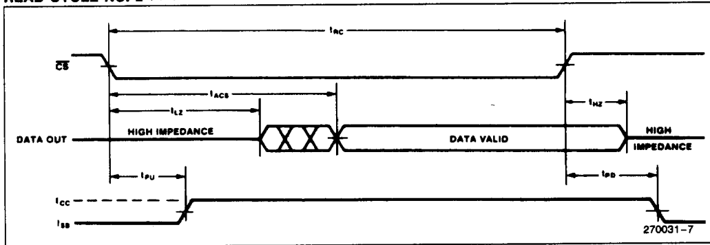
READ CYCLE NO. 2 (1, 3)
