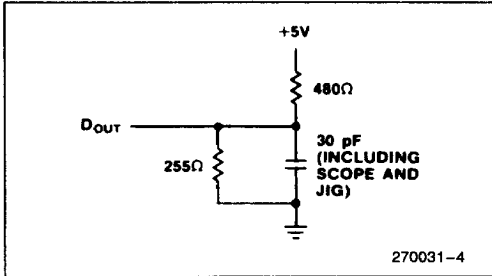
Load A
