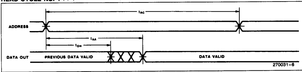
READ CYCLE NO. 1 (1, 2)
