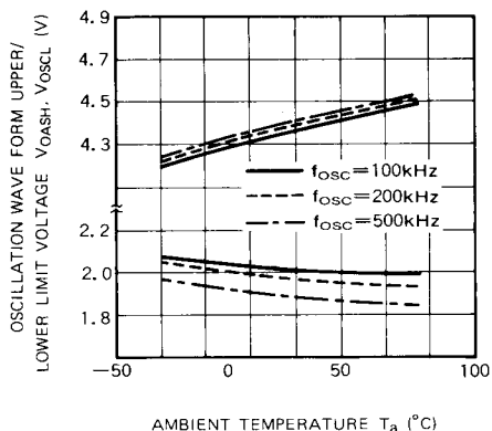
OSCILLATION WAVE FORM UPPER/LOWER LIMIT VOLTAGE VS. AMBIENT TEMPERATURE
