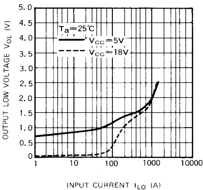
OUTPUT LOW VOLTAGE VS. INPUT CURRENT
