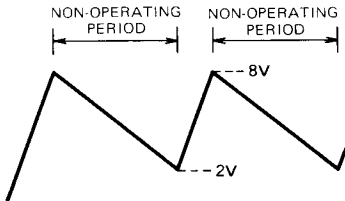
Figure 12 CT pin wave form
