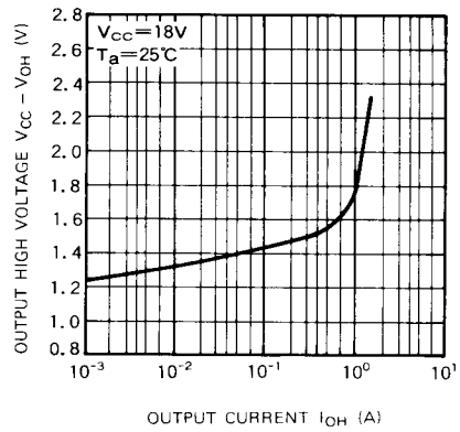
OUTPUT HIGH VOLTAGE VS. OUTPUT CURRENT
