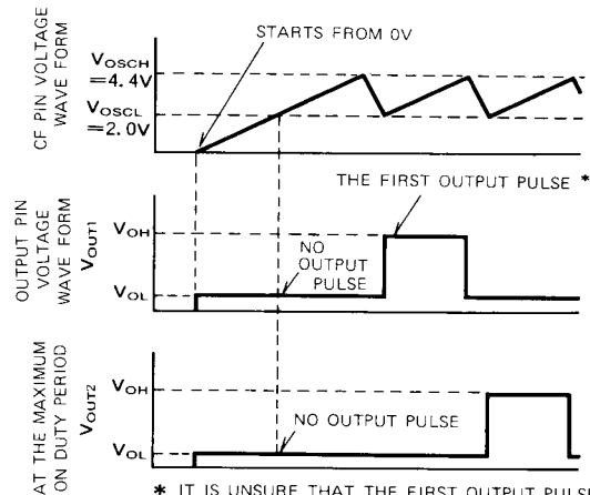
Figure 4 Relation between the oscillation wave form upon the activation and the output wave form
