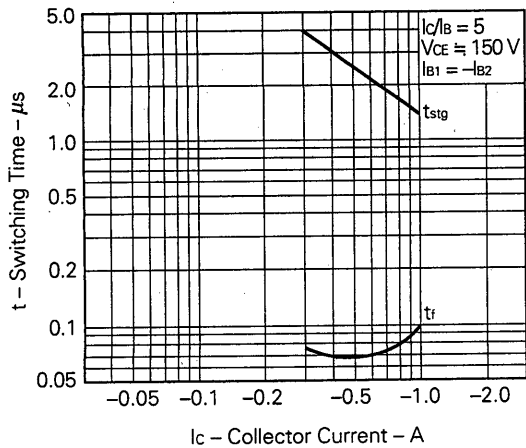
TURN-OFF TIME vs. COLLECTOR CURRENT
