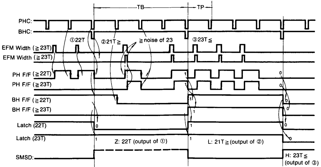
Fig. 22 When gain is 'H' in a speed-mode Timing Chart of SMDSD output
