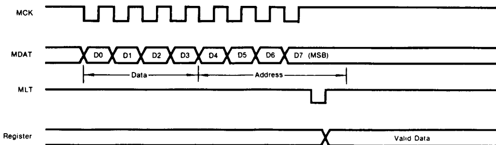
Fig. 6 Data Input Timing Diagram
