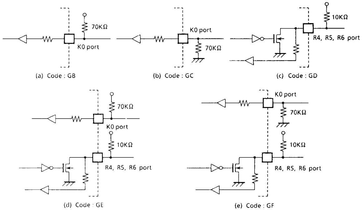
Figure 1-2. I/O code and external circuitry
