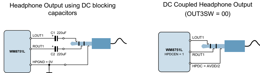
Figure 26 Recommended Headphone Output Configurations
