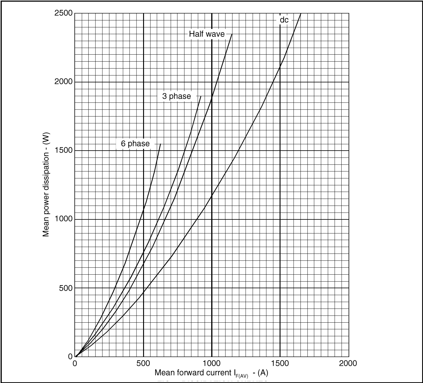
Fig. 2 Dissipation curves
